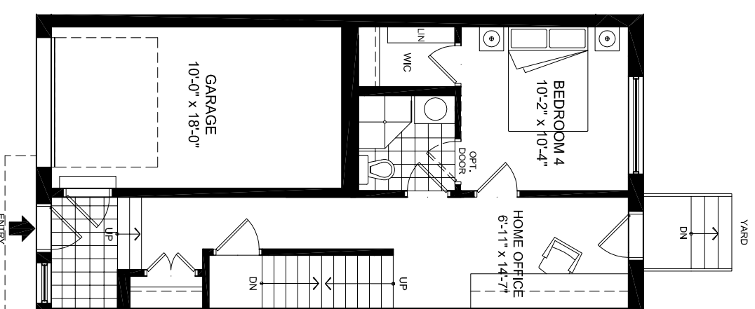
ENTRY LEVEL (OPTIONAL 4 BEDROOM PLAN) 490 SQ.FT.
