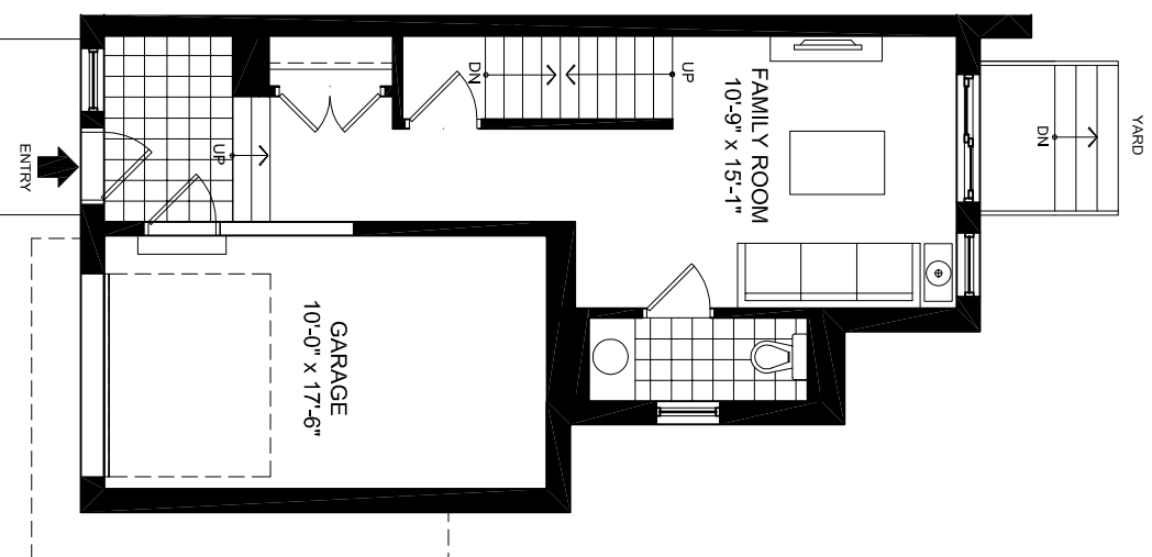
ENTRY LEVEL 403 SQ.FT.
