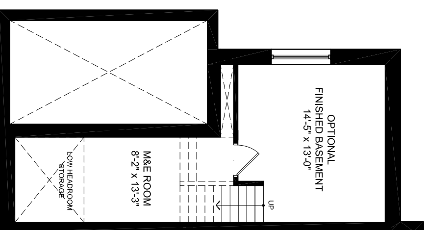
LOWER LEVEL 233 SQ.FT.
