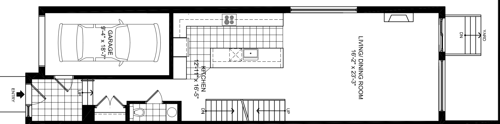
MAIN FLOOR PLAN 881 SQ.FT.
